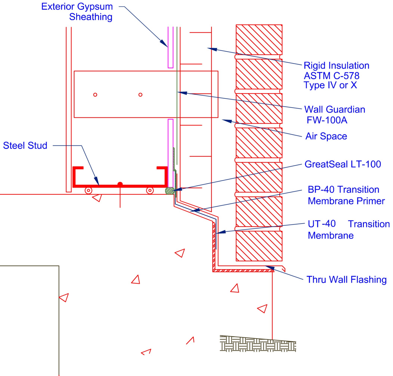
FOUNDATION DETAIL Wall Guardian FW-100-A System Not to scale
