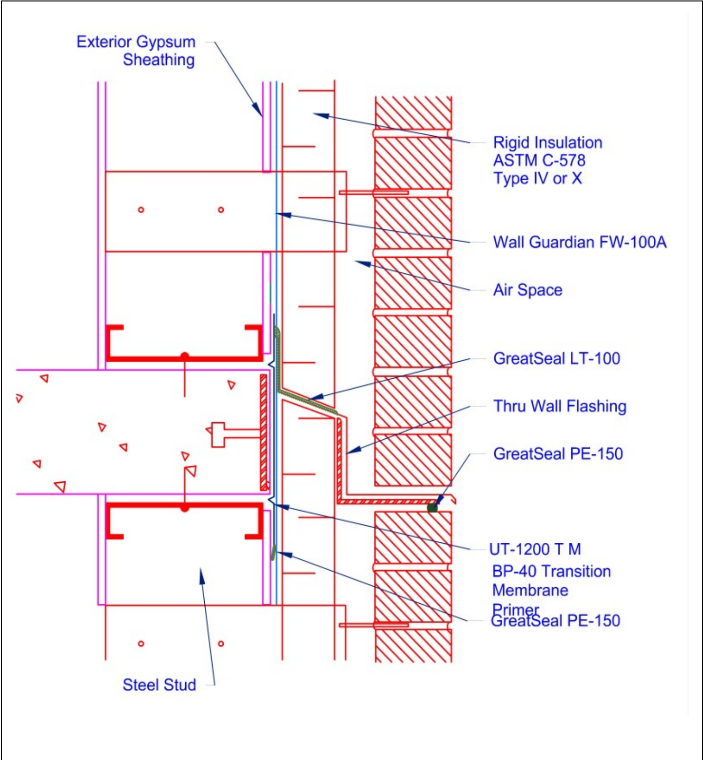
ANGLE DETAIL Wall Guardian FW-100-A System Not to scale
